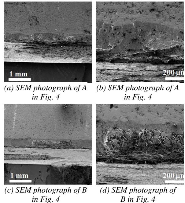
Fig. 5 SEM photograph of spalling failure parts
