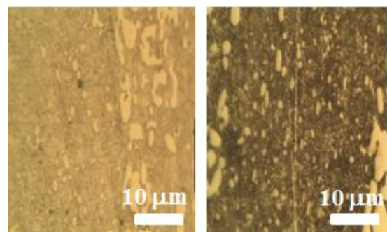
Fig. 6 Microstructure observation of spalling failure part and base metal
