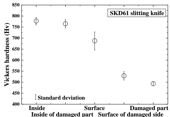
Fig. 9 Vickers hardness according to specimen conditions
