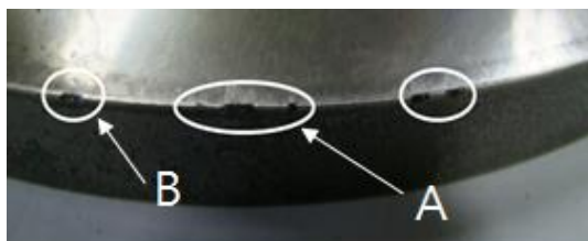
Fig. 4 Spalling failures at the slitting knife edge
