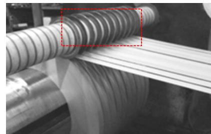
Fig. 2 Slitting process
