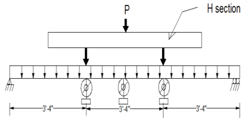
Figure 5: Loading setup for recording of deformation
