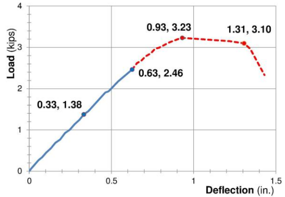
Figure 8: Deformation-Load relationship for first panel tested
