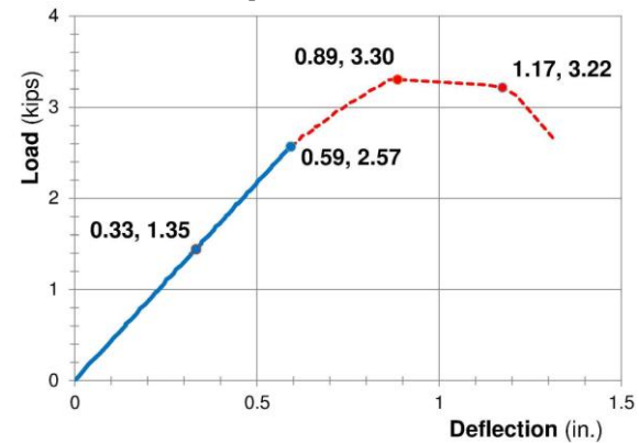
Figure 9: Deformation-Load relationship for second panel tested
