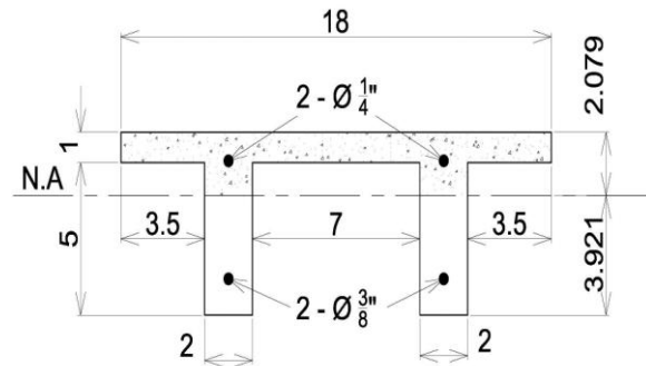
Figure 3: Cross-section of profiled concrete panel (Dimensions are in inches)
