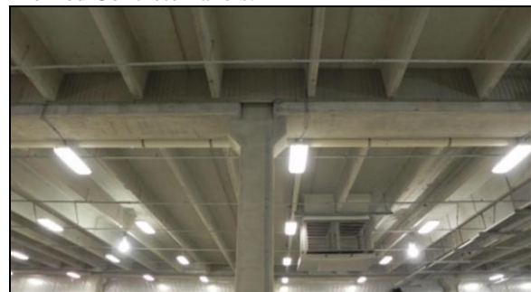
Figure 1: Use of Precast Profiled Concrete Panels as roof slab
