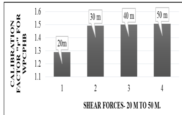
Figure 8: Calibration factor "r" with WPCPHB (S.F.) for spans- 20 to 50 meter
