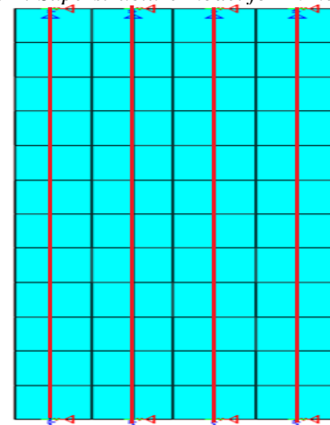
Figure 2: Superstructure model for 30meter span
