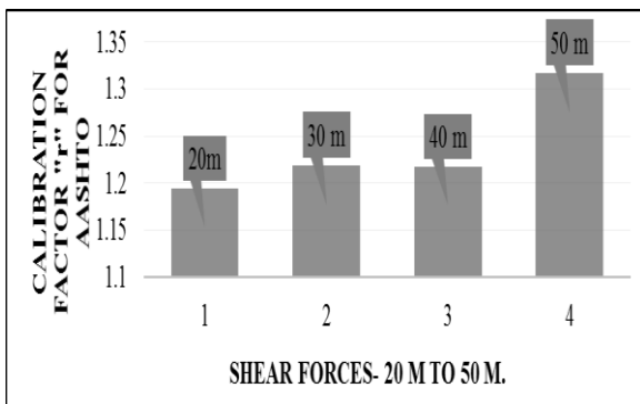
Figure 6: Calibration factor "r" with AASHTO (S.F.) for spans- 20 to 50 meter
