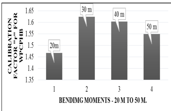
Figure 7: Calibration factor "r" with WPCPHB (B.M.) for spans- 20 to 50 meter
