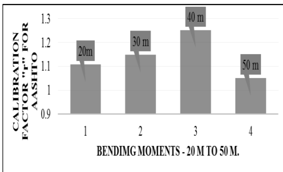
Figure 5: Calibration factor "r" with AASHTO (B.M.) for spans- 20 to 50 meter
