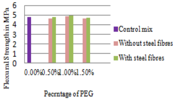
Figure 9 Flexural Strength-28 Days
