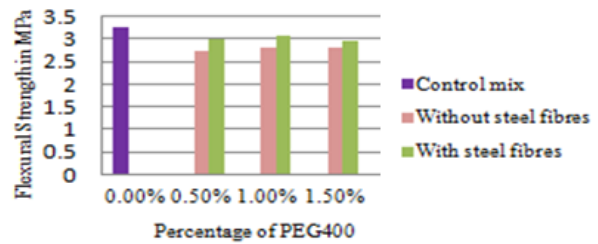
Figure 7 Flexural strength-3 days
