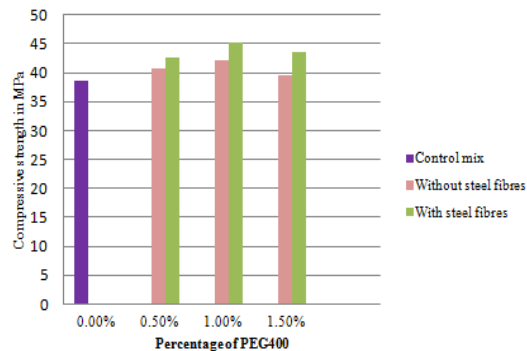
Figure 2: Compressive Strength-7 Days
