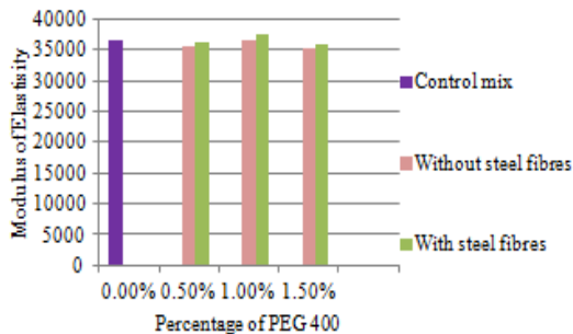
Figure 10 Modulus of Elasticity- 28 Days
