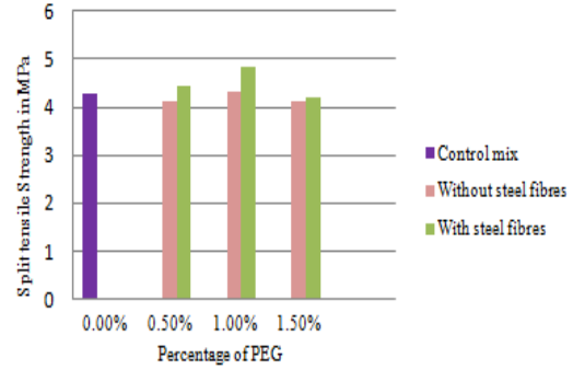
Figure 6 Split Tensile Strength-28 Day
