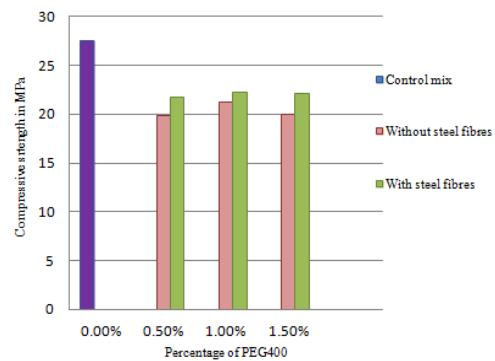
Figure 1 Compressive Strength-3 Days
