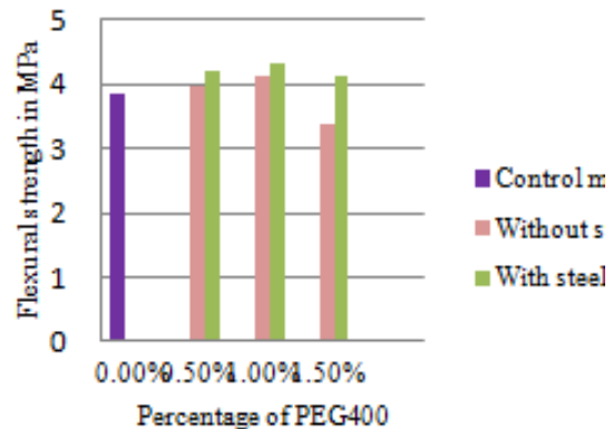
Figure 8 Flexural Strength-7 Days
