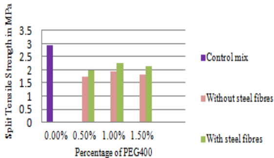
Figure 4 Split Tensile Strength-3 Days
