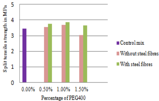
Figure 5 Split Tensile Strength-7 Days
