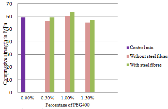
Figure 3 Compressive Strength-28 Days
